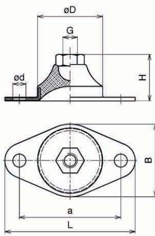
elasto-Flex-Elements Type 90
